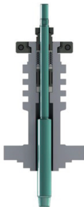
EXTENSION BONNET
